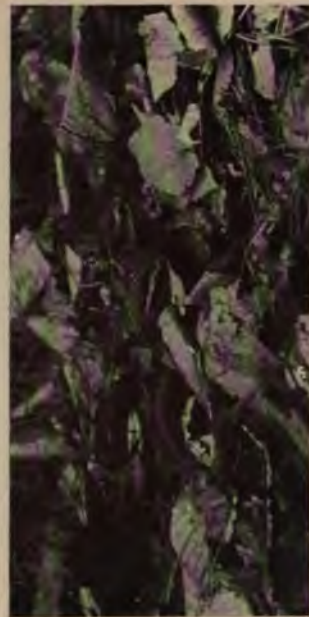
FIG. 93. Chipmunk ( Tamias striatus ) among dead leaves, its stripes picturing sticks or leaf-edges and shadows. (These picture-patterns are, of course, based on perfect obliterative shading.) Photographed from life, outdoors. (Captive chipmunk.)
